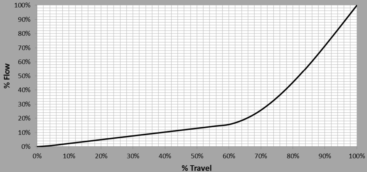
Typical Flow Profile Low Flow Control Valves
