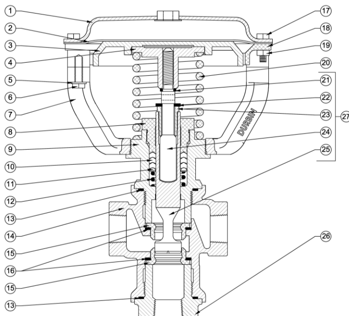
1/2"-2" 3W NC HARD SEATED PARTS LIST
