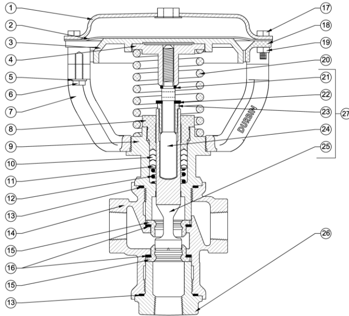
1/2"-2" 3W NC HARD SEATED PARTS LIST
