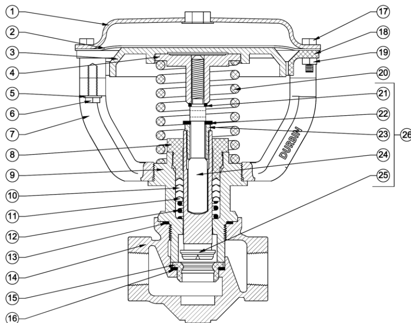
1/2"-1-1/2" 2W NO HARD SEATED PARTS LIST
