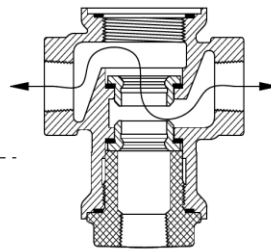
INLINE PORTING
