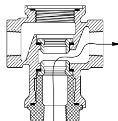
ANGLE PORTING
