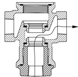
ANGLE PORTING
